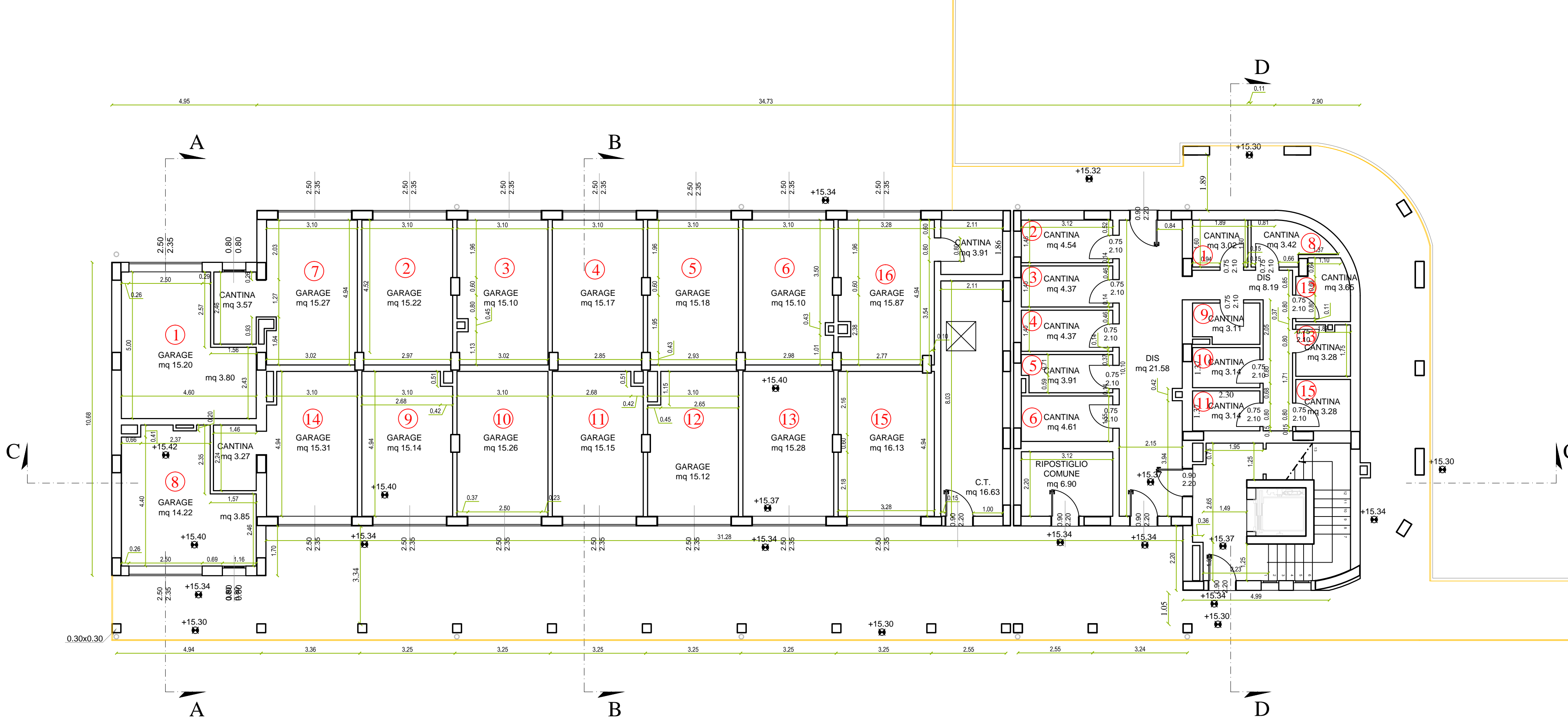
PIANO TERRA
